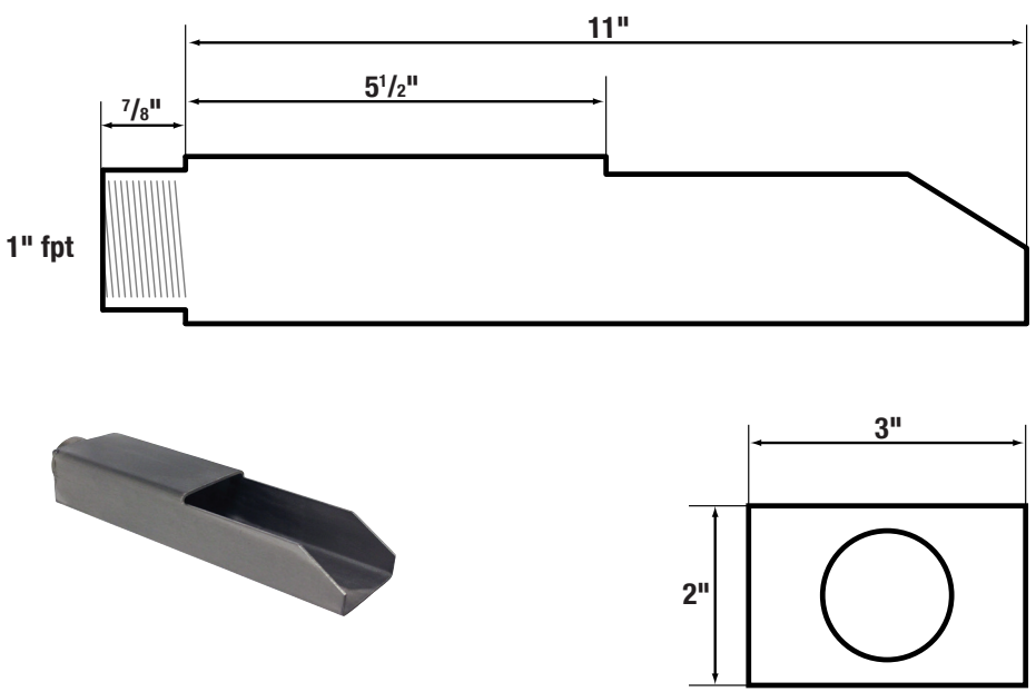
SWS3RN — rectangle channel wall scupper
