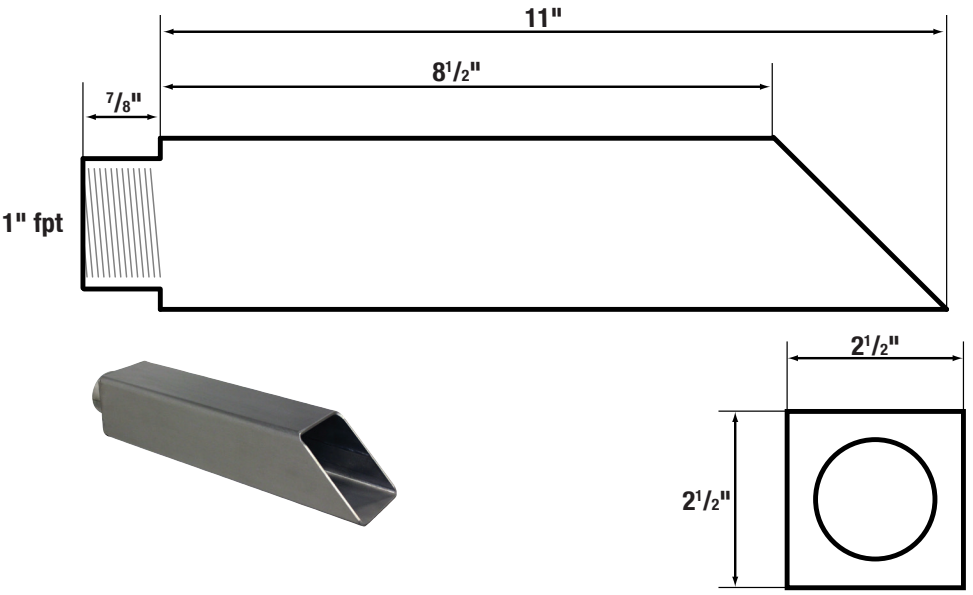
SWS2SN — 2½" square wall scupper
