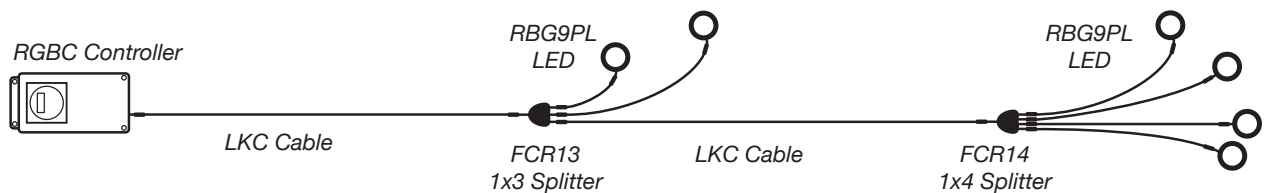
RGBC Controller with Remote Control
