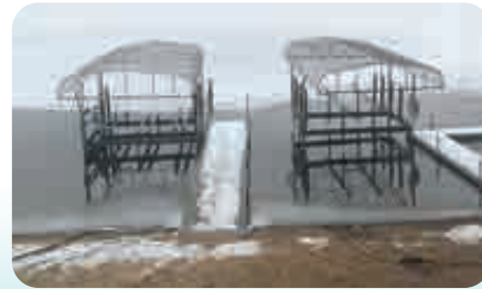
Two 60 watt KLC compressors keep the docks and boat lifts shown ice-free for less than $10 per month!
